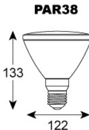
Dimensional Drawings
