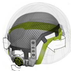
1. Nape dial to adjust circumference
