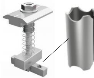
Mid Clamp with Ground Pins
