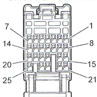
Green BCM Connector X3 Pinout
