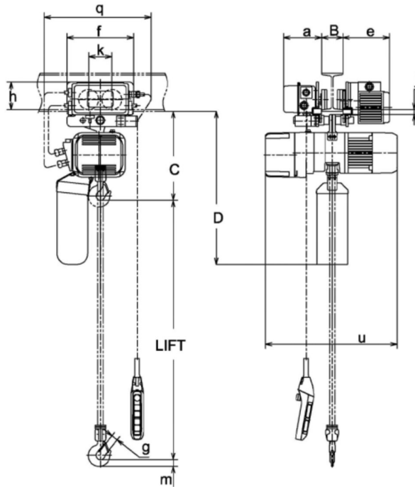
Single Fall ER2M Adjustable 2-speed; *For informational purposes only, contact KITO for dimensional drawing
