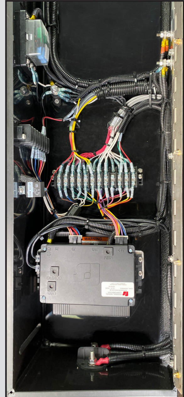
UNDER BACKSEAT REAR WIRING
