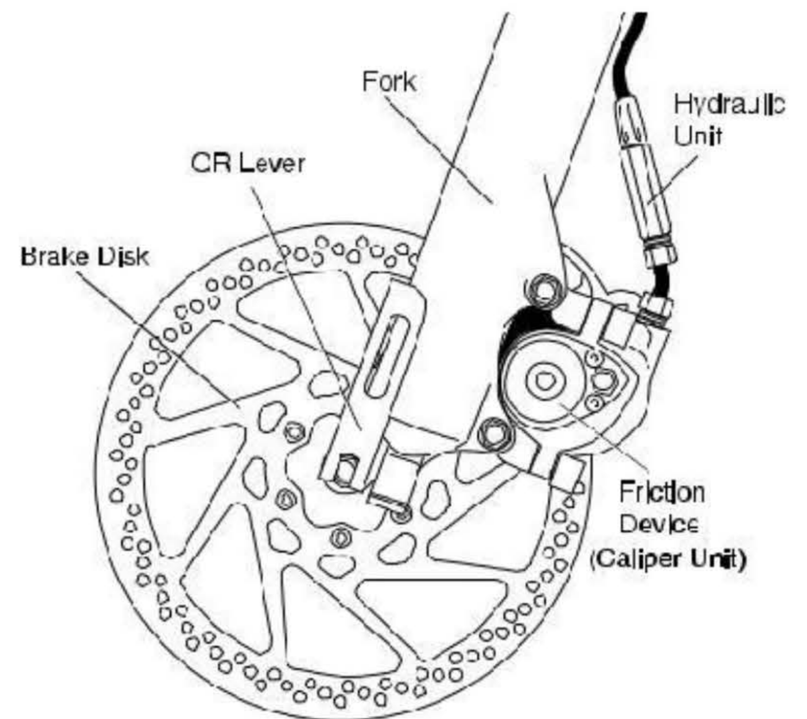
Disc Style Brake System
