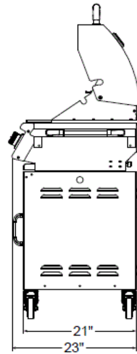
RIGHT VIEW
