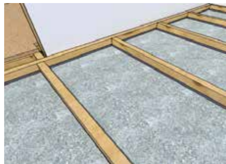
Fig. 2 Concrete Installation
