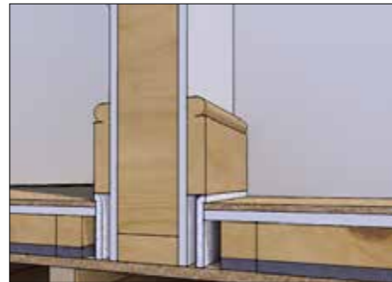
Fig. 5 Timber Installation
