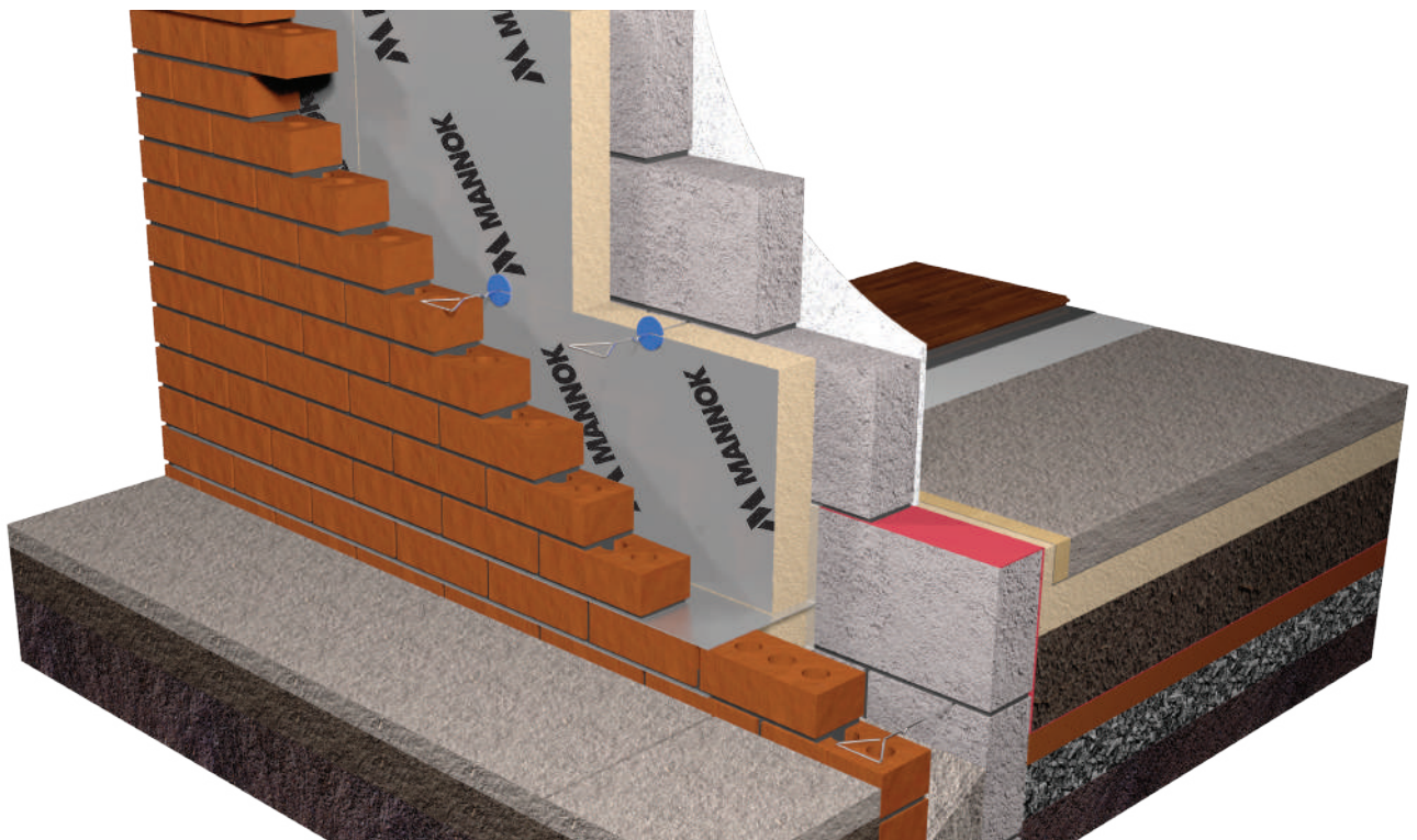
Cavity walls: MC in masonry - partial fill
