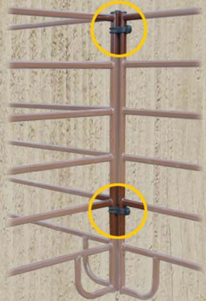
HB672 - 16 ga. showing 3-way Panel with Flex Strap
