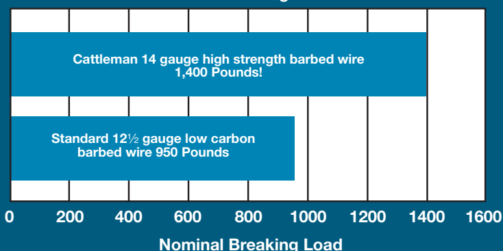
Wire Strength
