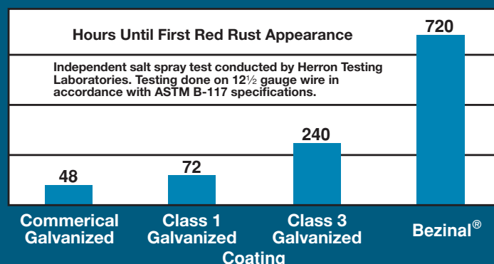
Corrosion Resistance
