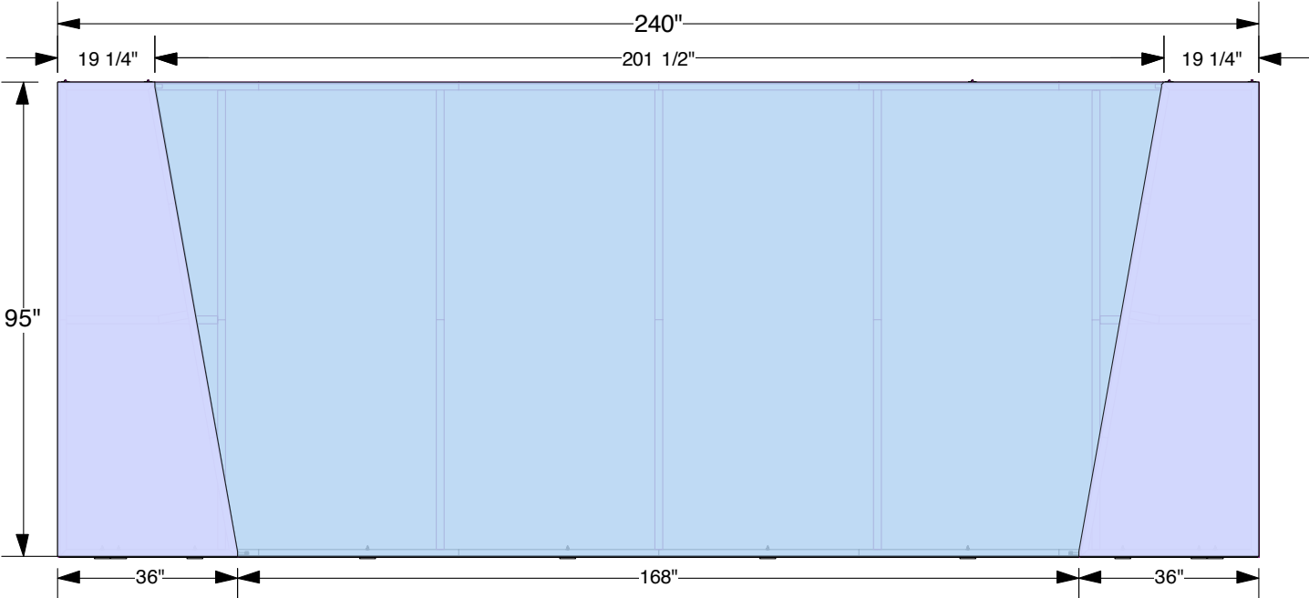
FRONT VIEW
