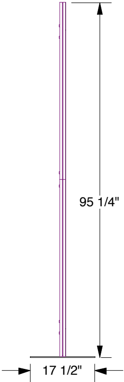
RIGHT VIEW
