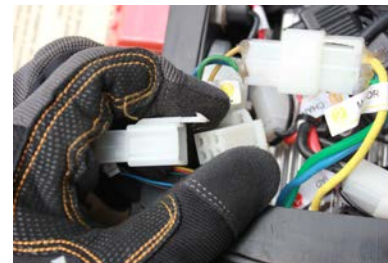
A3. Unplug the connector with '2. motor' and '3. hall sensor', then try to check if there is anything bended. Adjusted them if needed or bend it a bit to create a better contact.
