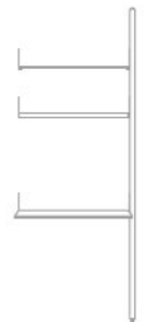
Branch Desk Unit Add-On W31.5 D11.5/20.5 H84 (in) W79 D29/52 H213 (cm)
