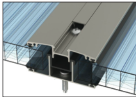
Cod. 4891 Upper Aluminum Profile with Hidden Screw 2/25
