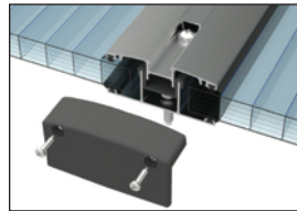
Cod. 4898 Poli-Lok Plug
