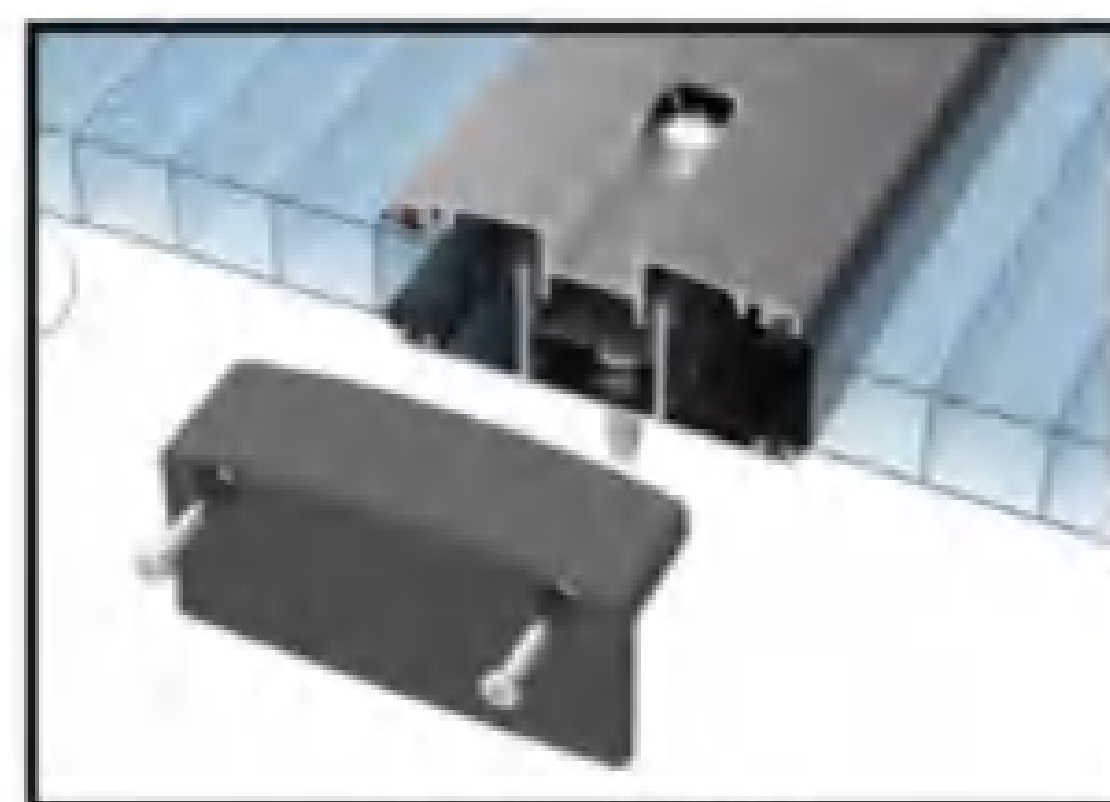
Cod. 4898 Poli-Lok Plug using #10 by 1" fastener
