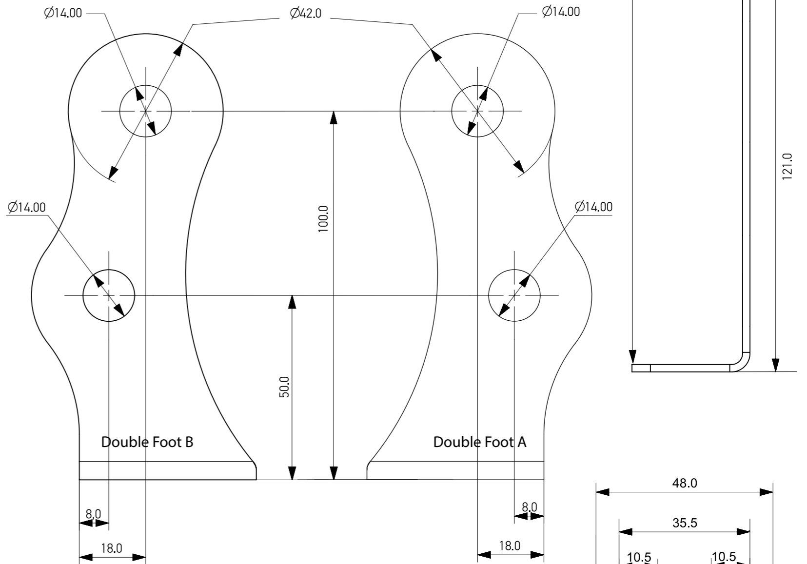
DOUBLE 50/100MM STAINLESS STEEL MOUNTING BRACKET
