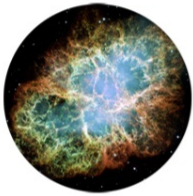
Crab Nebula
