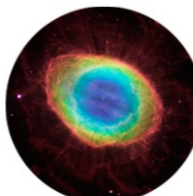
Ring Nebula
