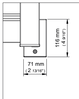
Ingombro placchetta a muro Wall-plate dimensions Dimensions de la plaque
