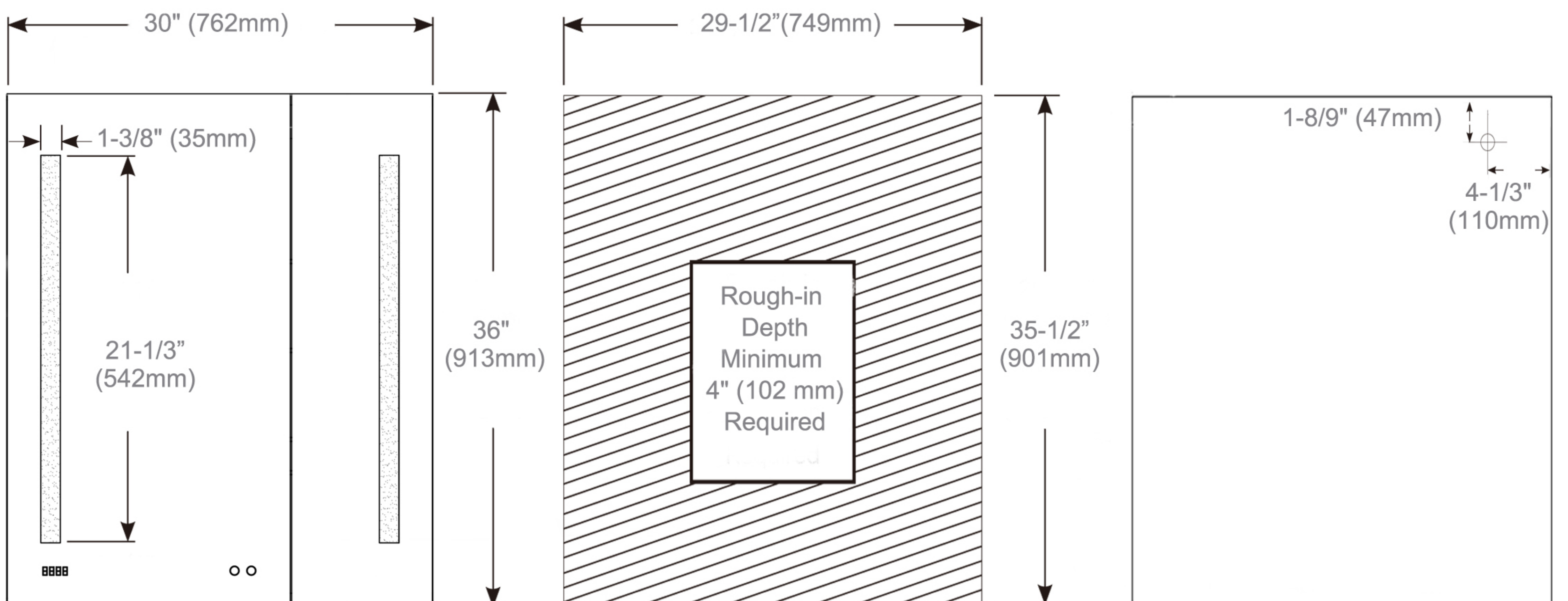
Cabinet Dimensions
