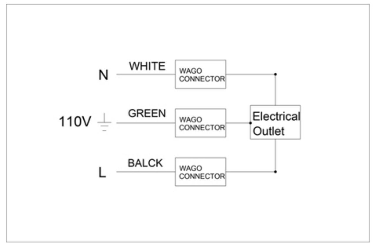
Circuit Diagram
