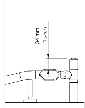
Ingombro frontale valvola Cylinder Valve Cylinder frontal dimension Dimension frontale de la valve Cylinder
