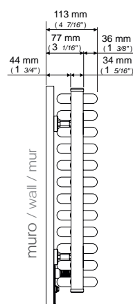
Ingombro con attacco corto Measurements with short wall brackets Mesurations avec attache court
