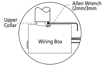
Fig. 4: Mounting of W2xxC Series Towel Warmers
