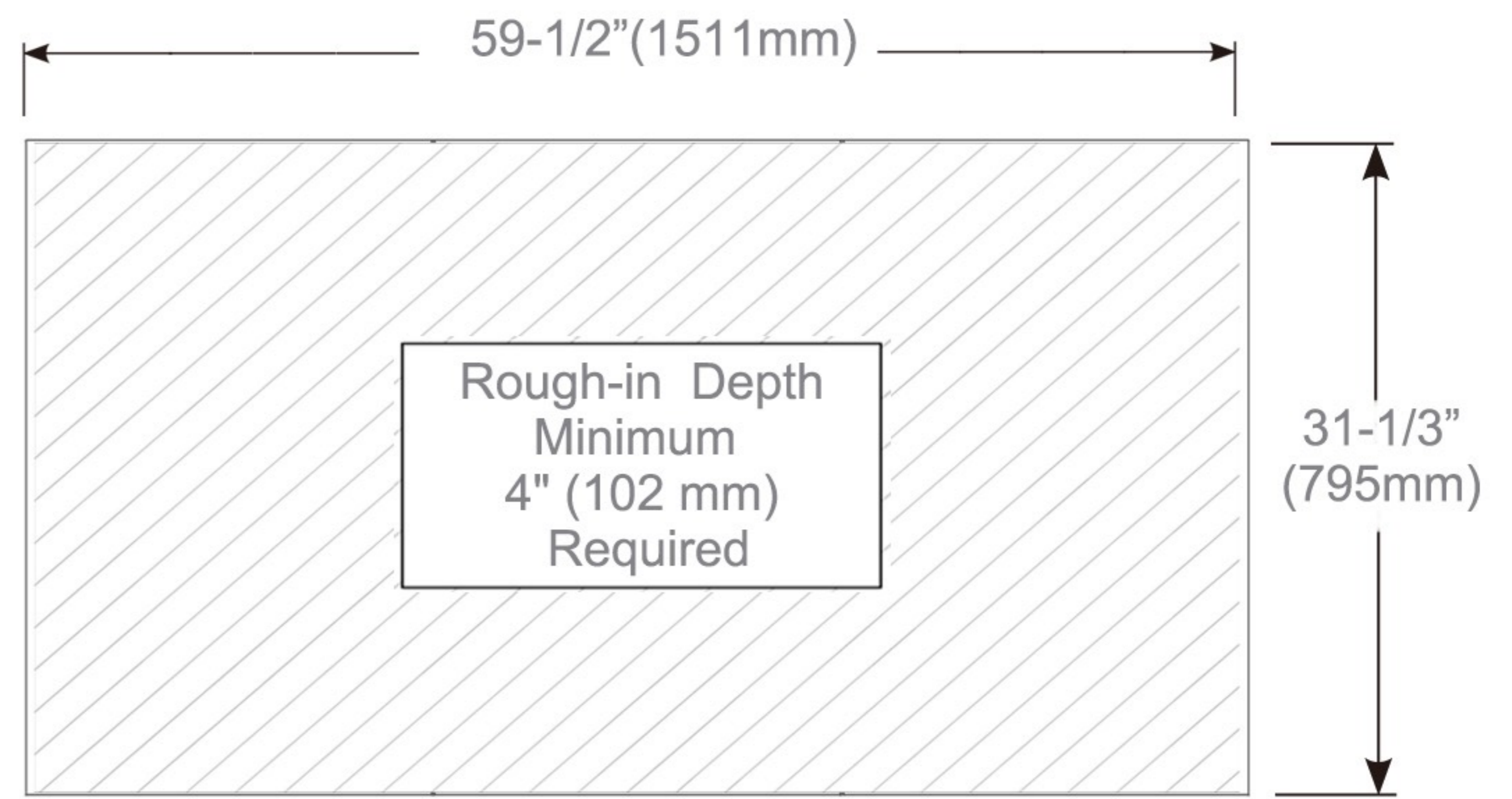
Rough-in Dimensions
