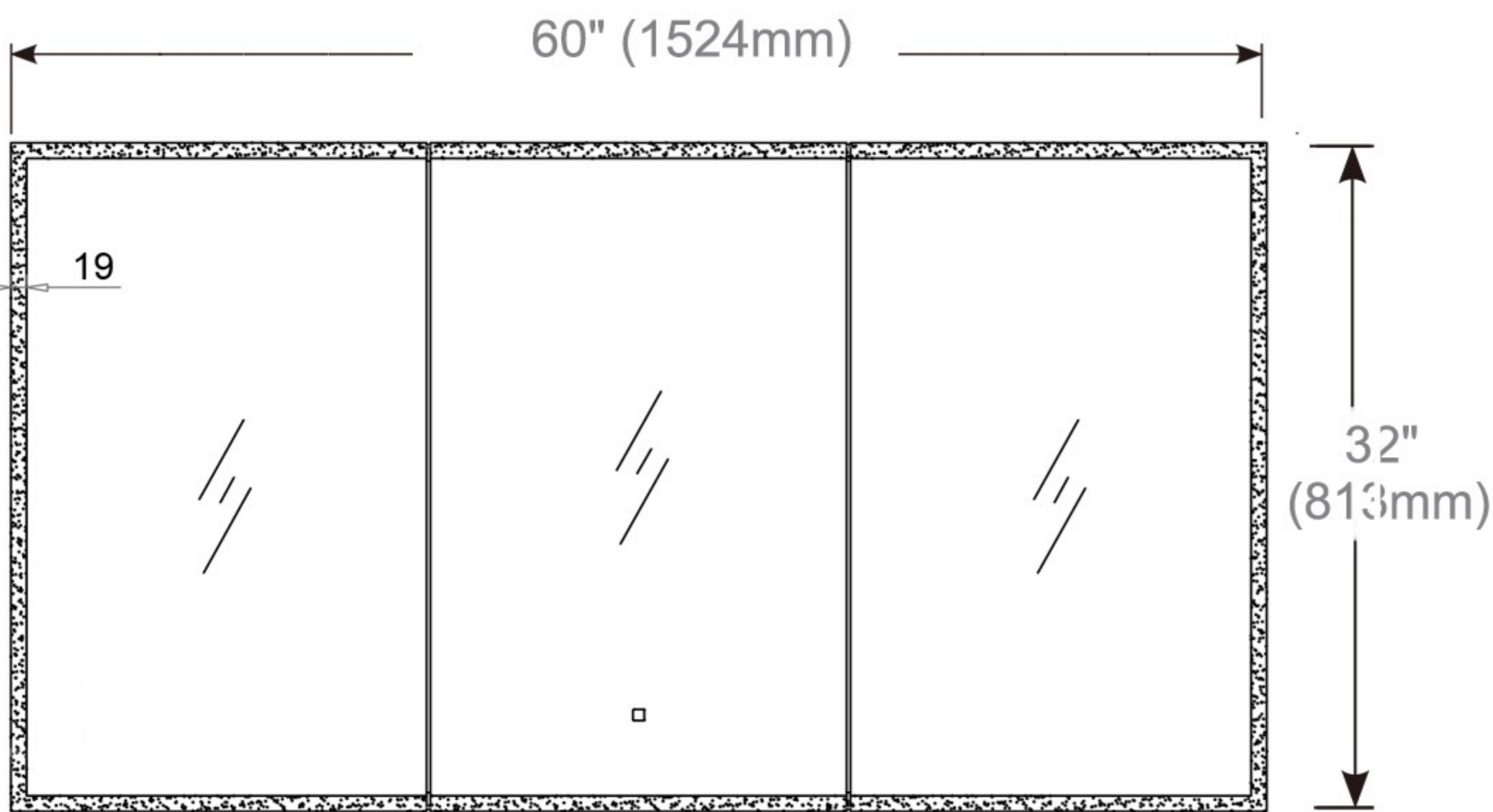
Cabinet Dimensions
