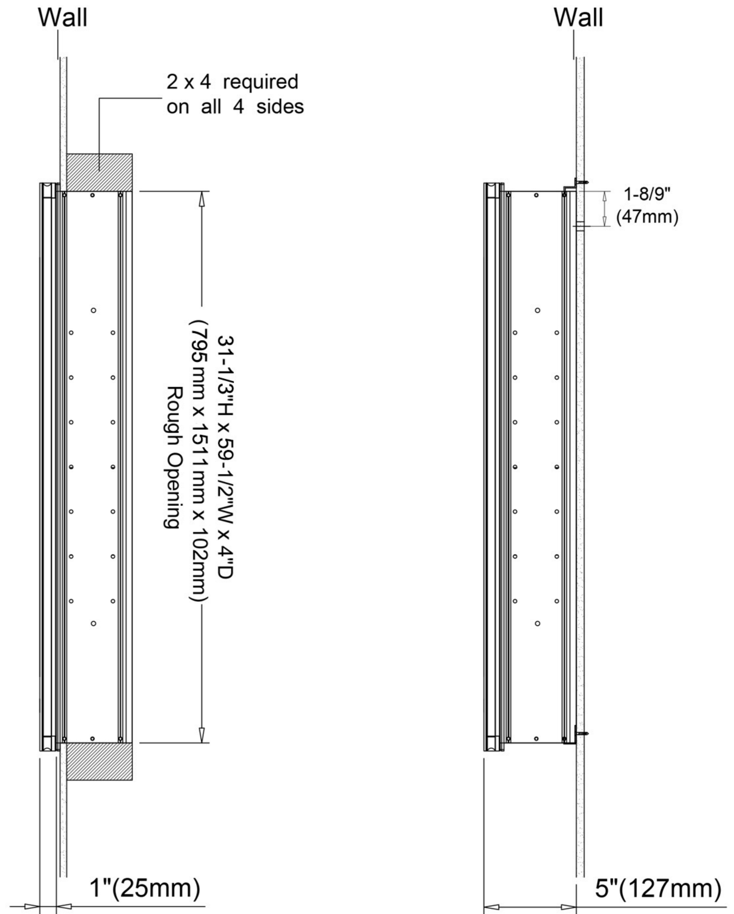
Recessed Mount
