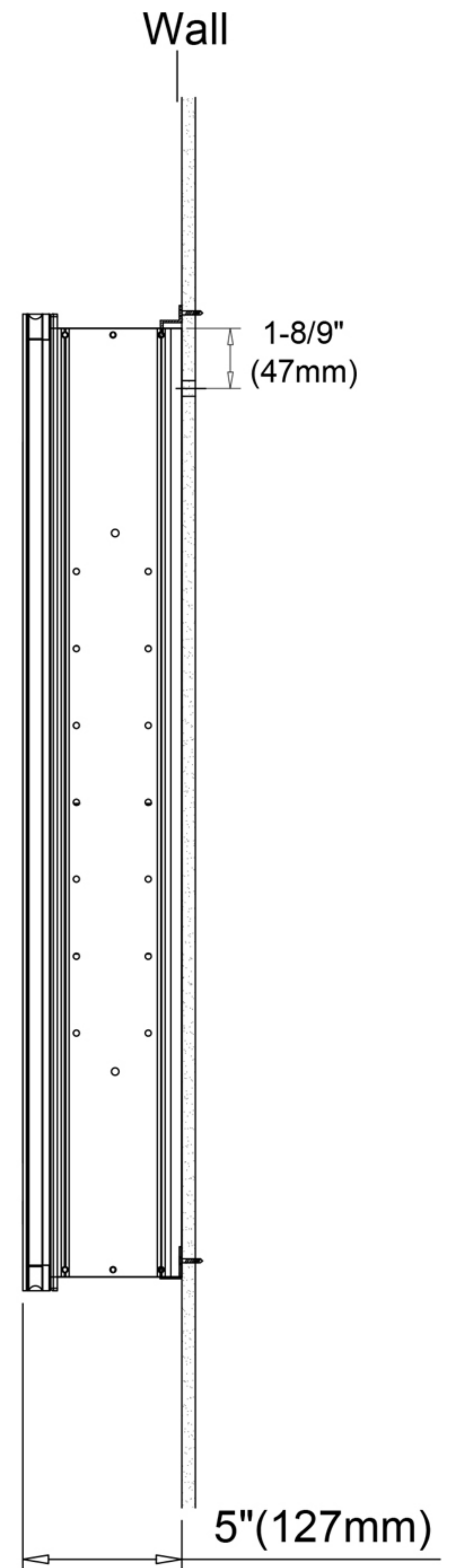
Surface Mount
