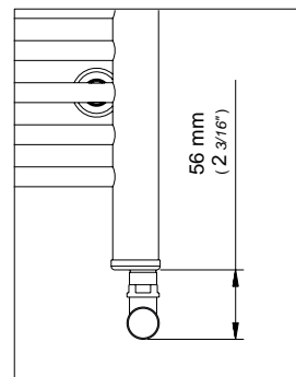
Ingombro valvola Cylinder Valve Cylinder dimension Dimension de la valve Cylinder
