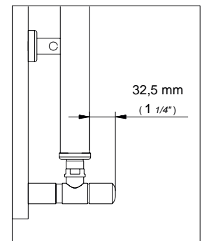
Ingombro frontale valvola Cylinder Valve Cylinder frontal dimension Dimension frontale de la valve Cylinder
