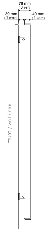
Ingombro con attacco corto Measurements with short wall brackets Mesurations avec attache court
