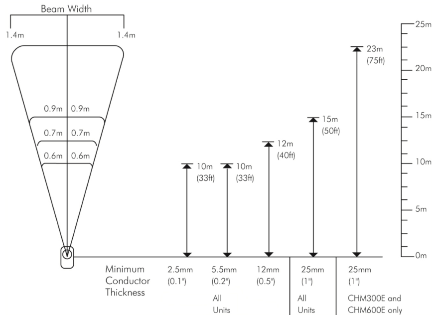
CHM Range versus Cable Thickness
