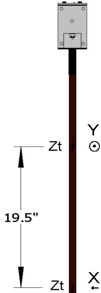
Figure 1: Sensor Location
