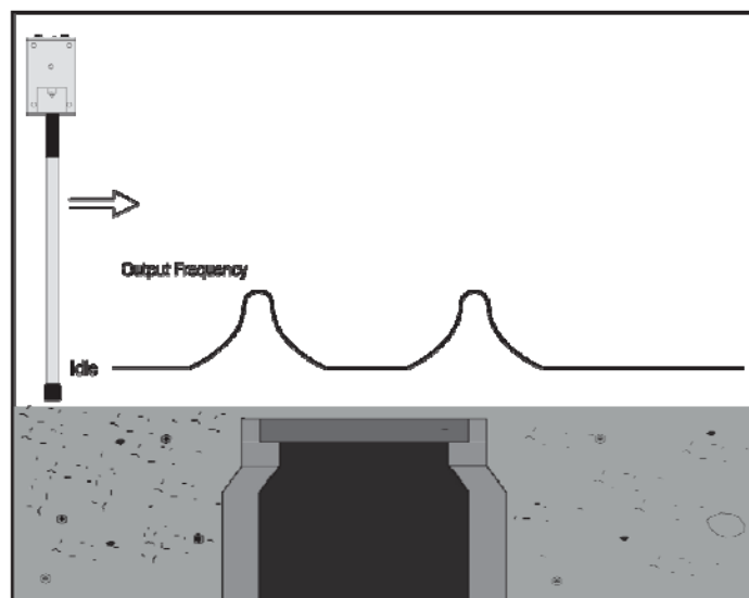
Figure 9: Manhole Cover
