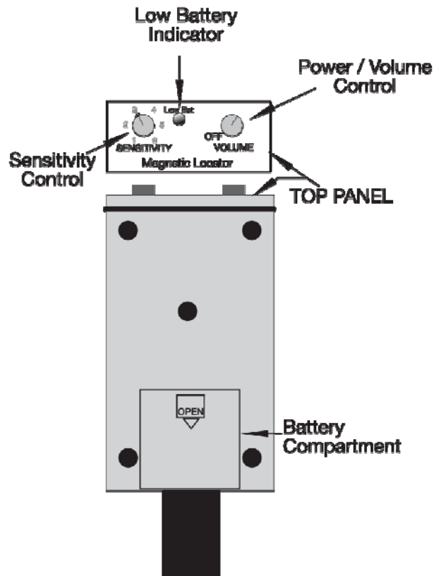
Figure 2: Instrument Controls
