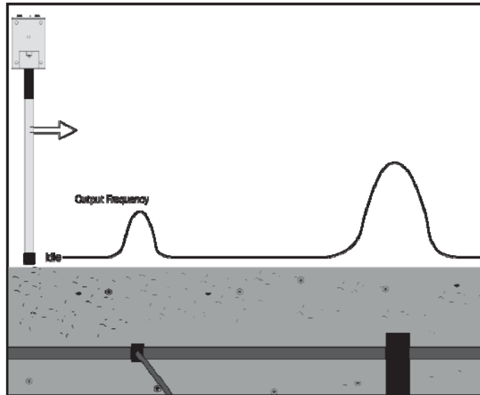
Figure 7: Service Connections & Valve Boxes
