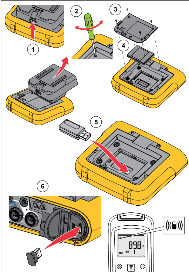
Figure 1. Adapter Installation
