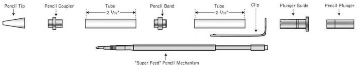
Diagram B: PENCIL PARTS
