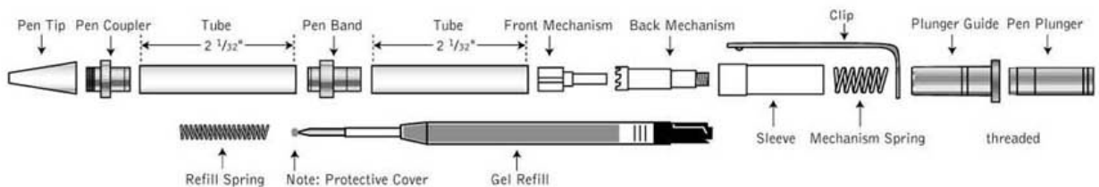
Diagram A: PEN PARTS
