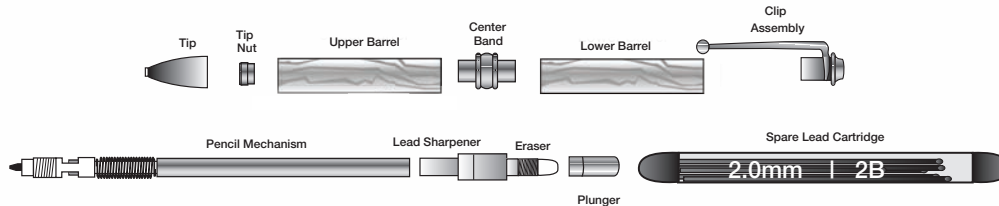
DIAGRAM E • Pencil Assembly
