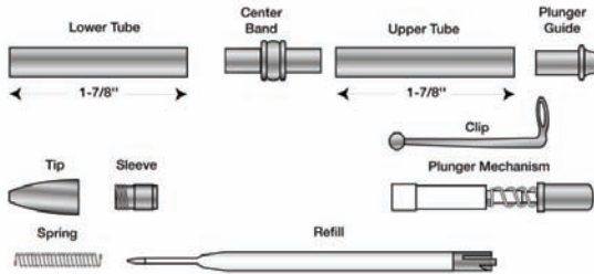
DIAGRAM A / Pen Parts list
