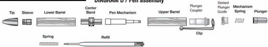
DIAGRAM D / Pen assembly
