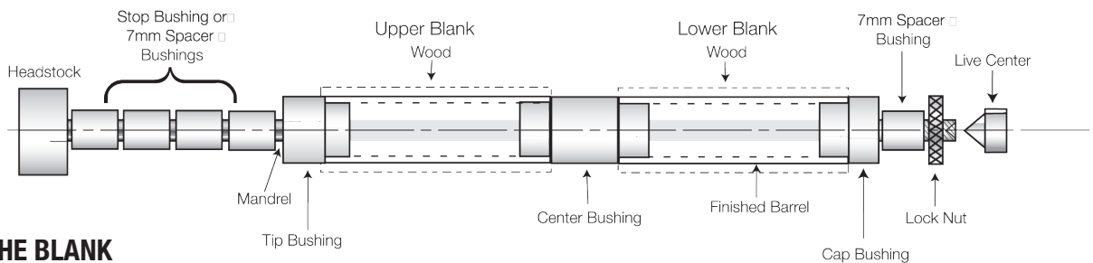
DIAGRAM C / Turning the blanks
