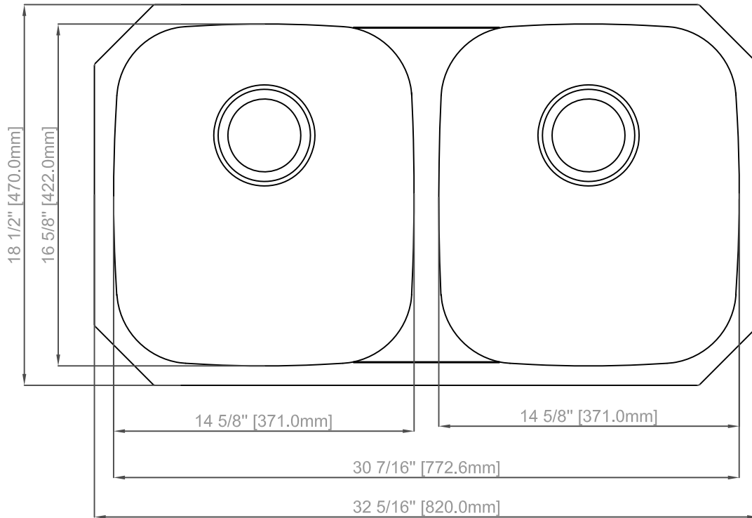
OVERHEAD VIEW
