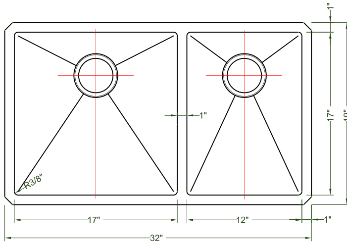
OVERHEAD VIEW
