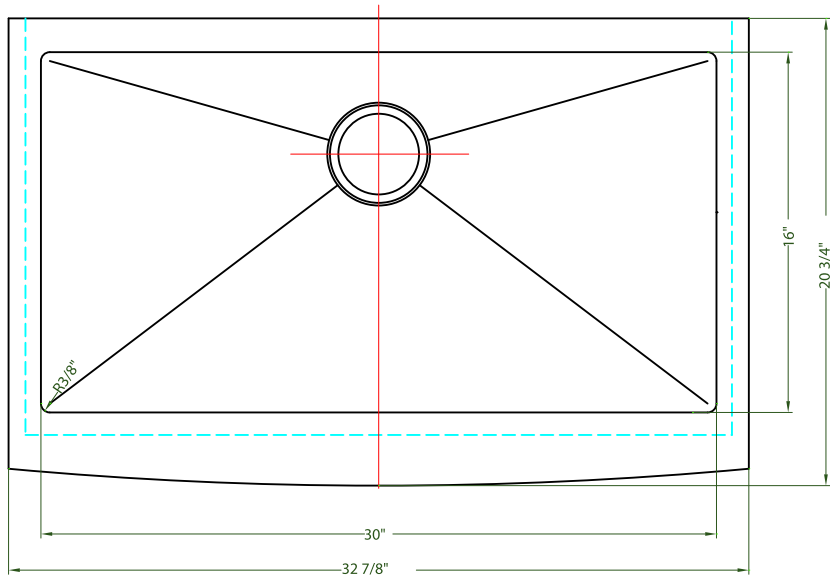
OVERHEAD VIEW
