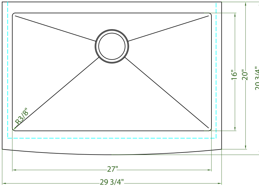
OVERHEAD VIEW
