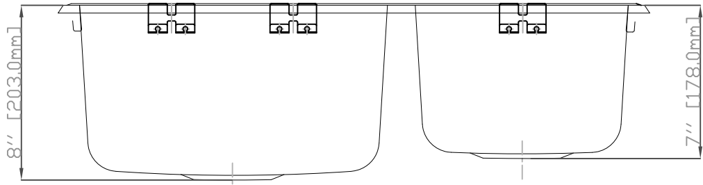
FRONT VIEW
