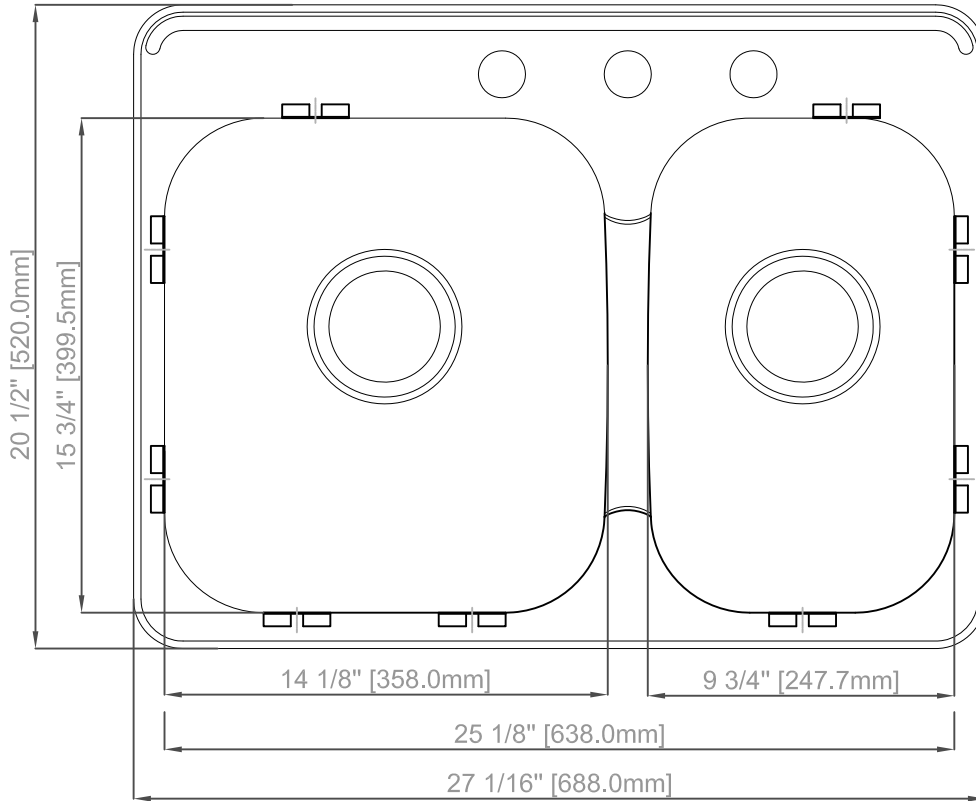
OVERHEAD VIEW
