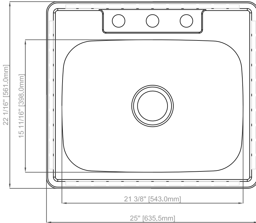
OVERHEAD VIEW
