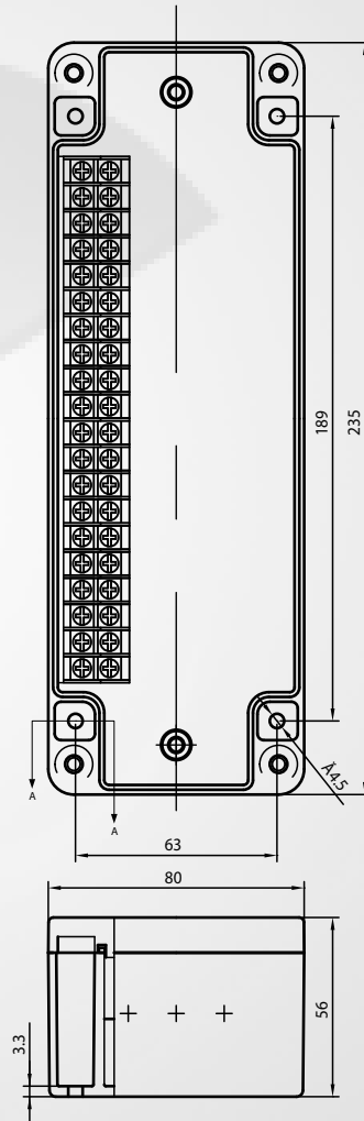
SECTION A - A SHOWN WITH COVER
