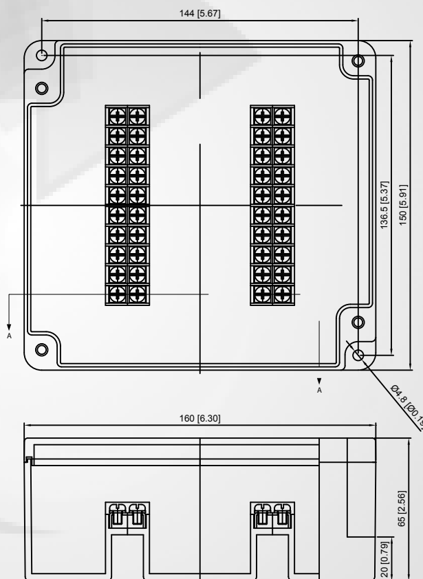
SECTION A - A SHOWN WITH COVER
