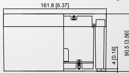
SECTION A - A SHOWN WITH COVER
