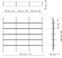
Wall fixing 3 modules Width: 279cm Depth: 33cm Height: 240cm
