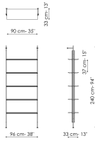
Wall fixing 1 module Width: 96cm Depth: 33cm Height: 240cm
