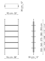
Ceiling fixing 1 module Width: 96cm Depth: 30cm Height: 255-265-275-285-295cm
