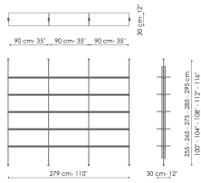
Ceiling fixing 3 modules Width: 279cm Depth: 30cm Height: 255-265-275-285-295cm
