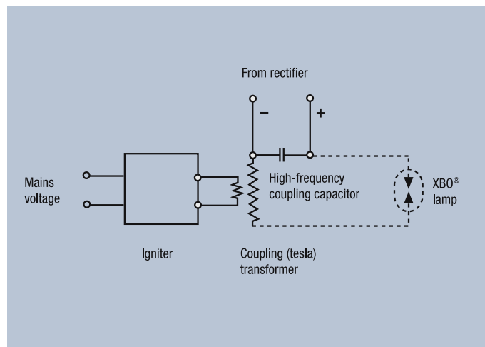
Fig. 19 Block diagram showing inductive coupling of high-frequency ignition pulses into the lamp circuit (superimposing igniter).
