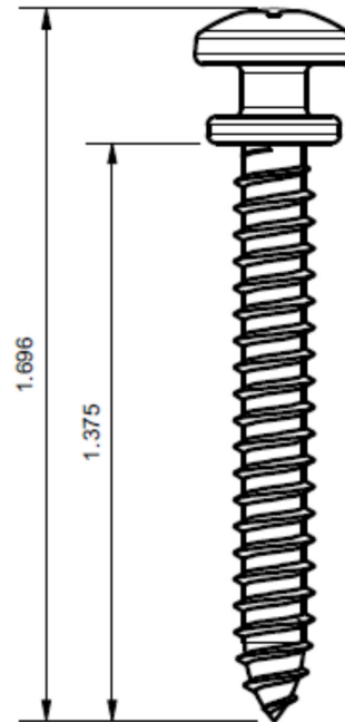
236 COMBINATION SCREW
