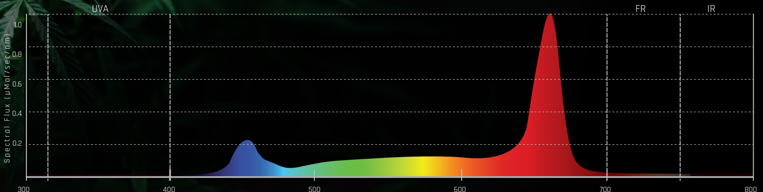
Spectral Quantum Distribution (SQD) Fohse™ A3i 1500W Plus+ Model FIXED SPECTRUM
