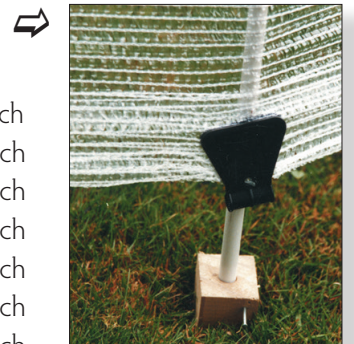
Butterfly clip fastening
