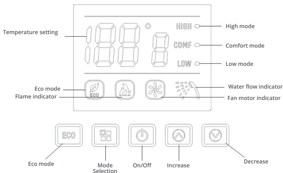
Control Panel Diagram
