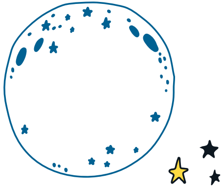
FULL MOON
