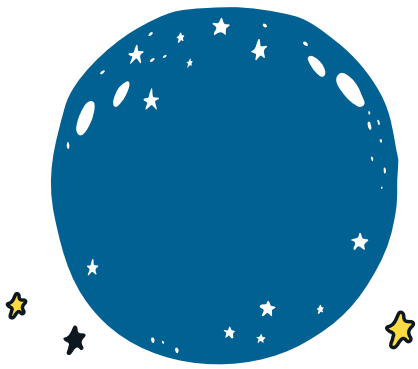
NEW MOON
