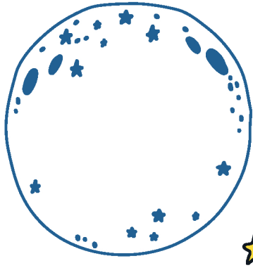
FULL MOON
