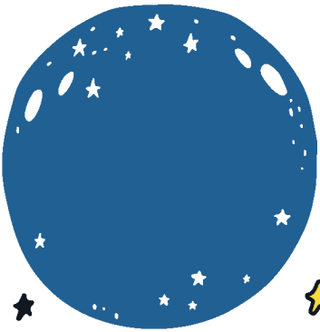
NEW MOON
